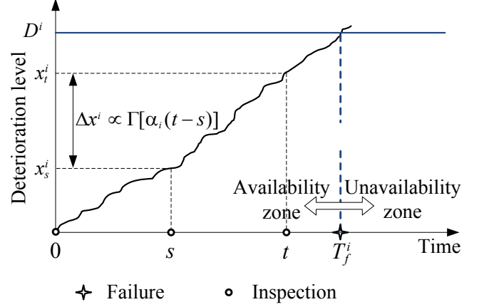
Figure 1. Description of the deterioration process (X_t^i)_{t \geq 0} for component i without maintenance activities.
