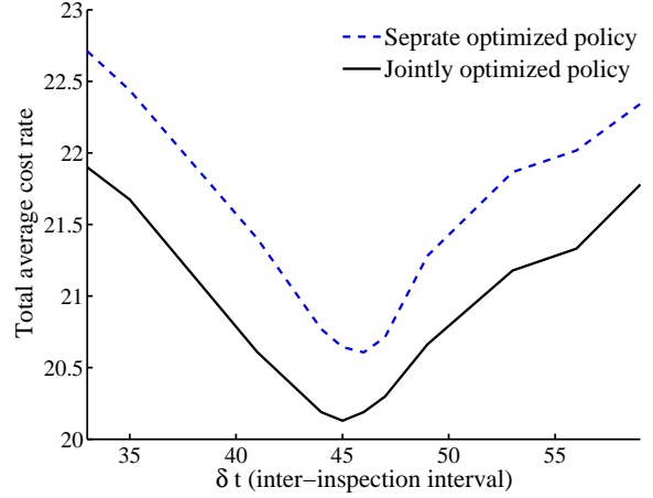
Figure 5. Relation of the total average cost rate between the joint and separate optimization.
