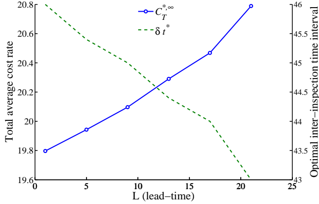
Figure 6. Influence of the lead-time on the proposed joint policy.
