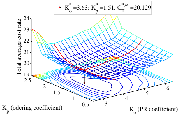
Figure 4. Cost surface of the proposed joint policy as a function of the K_p and the K_o considering at \delta t^* = 45 .
